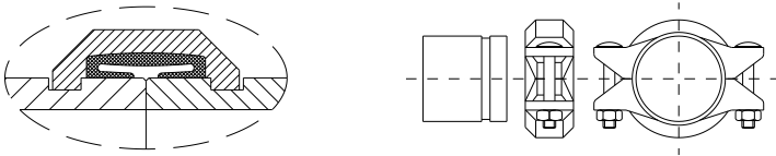
CONNESSIONE A GIUNTO FLESSIBILE (VICTAULIC) / FLEXIBLE COUPLING CONNECTION (VICTAULIC)
